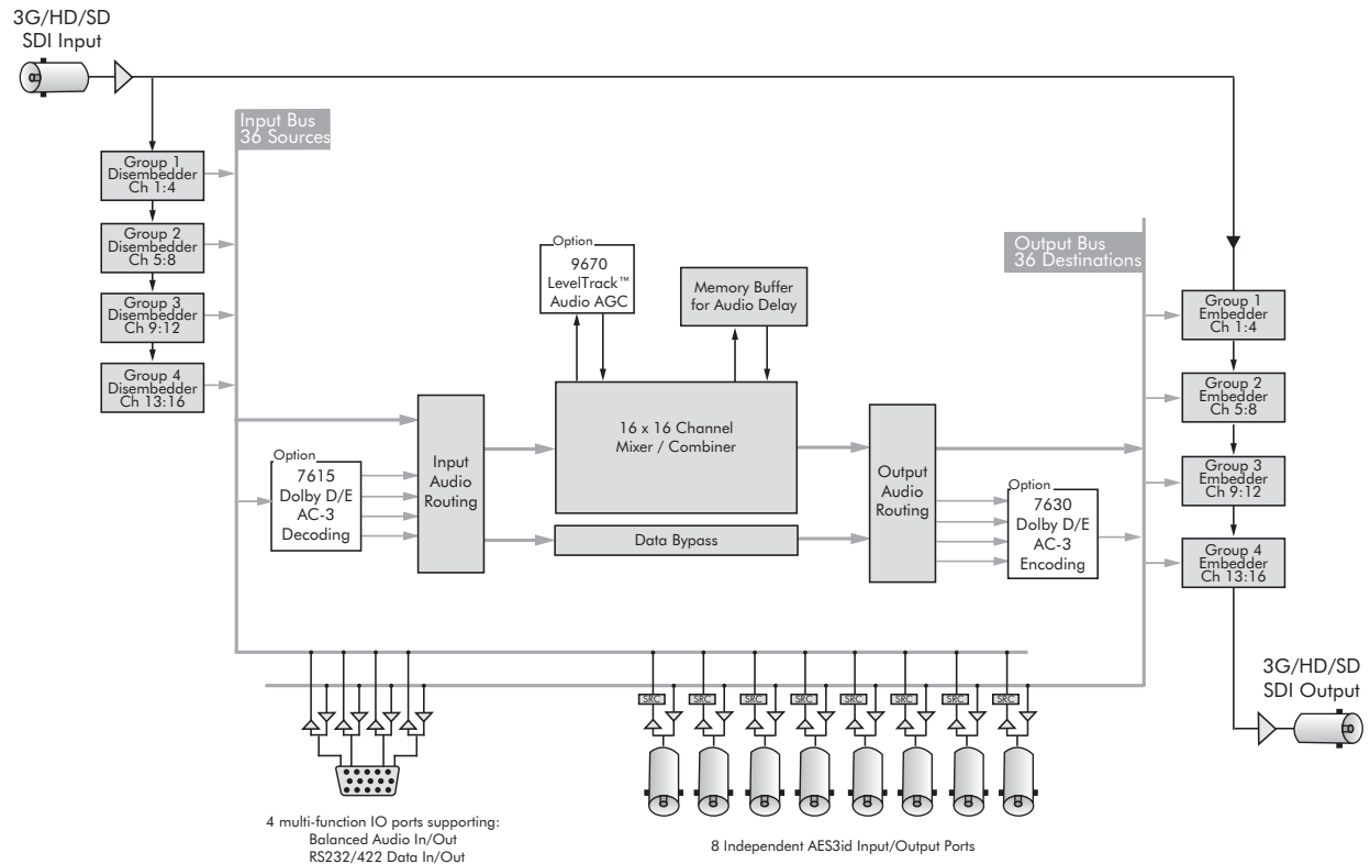
Avenue 9600 Functional Block Diagram
