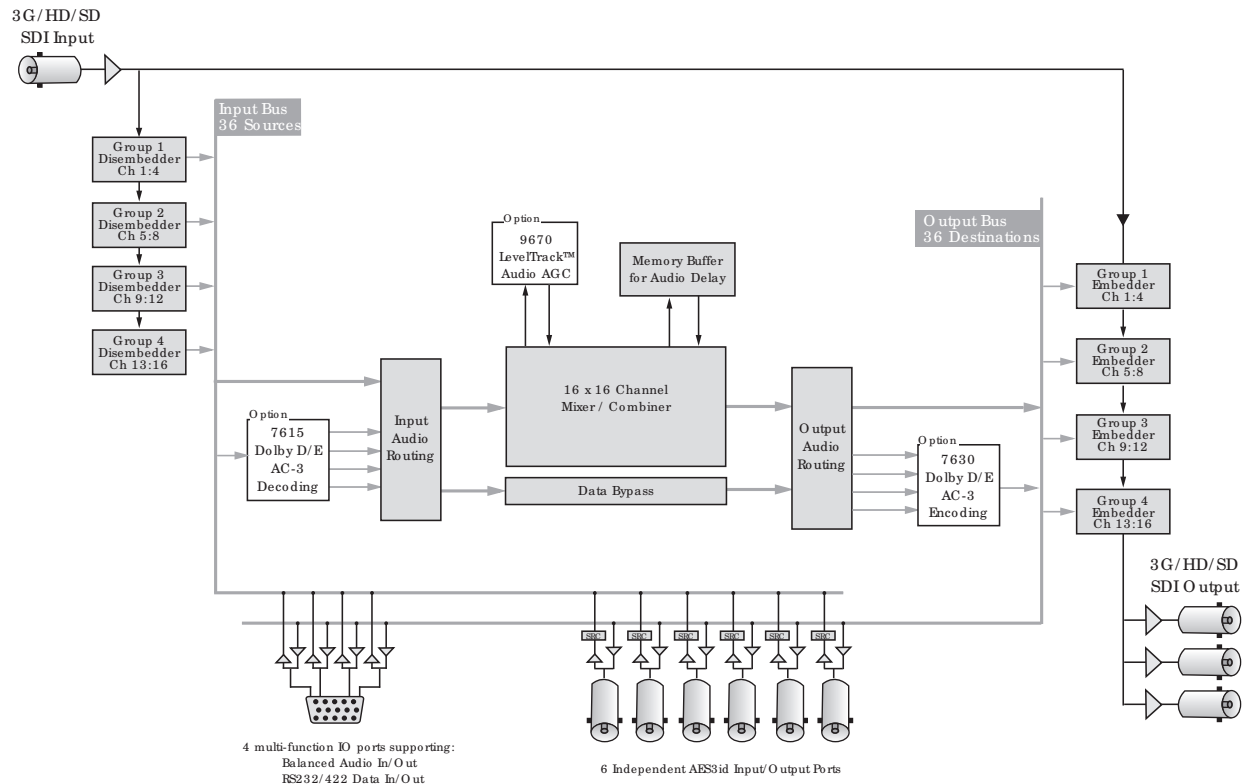
Avenue 9600-XV Functional Block Diagram
