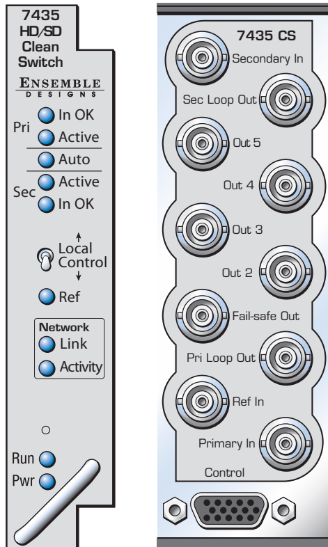
7435 Lexans: front, 3RU rear and 1RU rear
