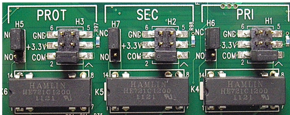
Close up of relay section and associated jumpers on the 9455 module
