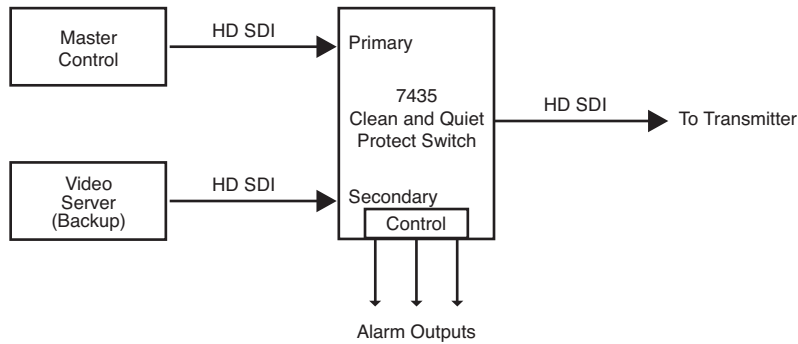
Redundant Auto-Switched Conversion with 7435 Module
