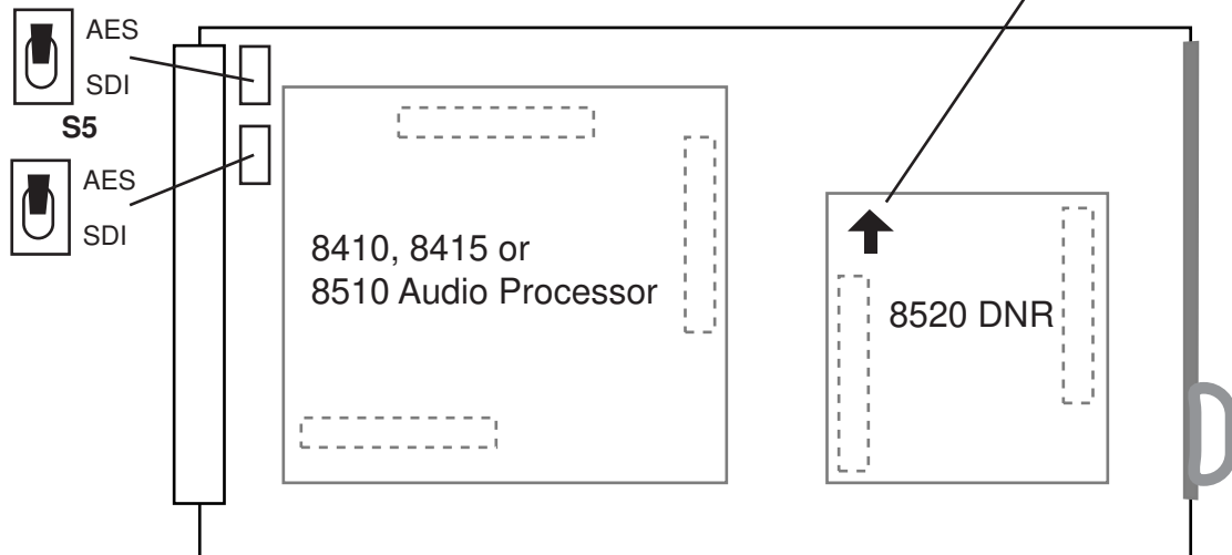
Configure Rear BNCs and Submodule Installation
