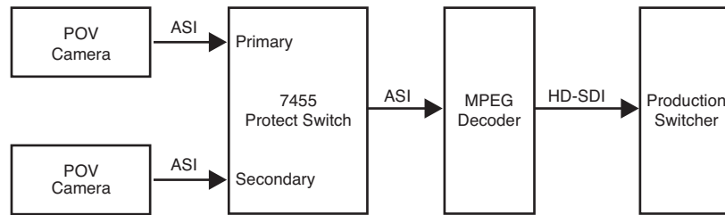
Signal Decision Maker With 7455 Module
