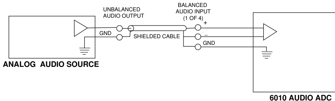
6010 Driven by Single-Ended (unbalanced) Source
