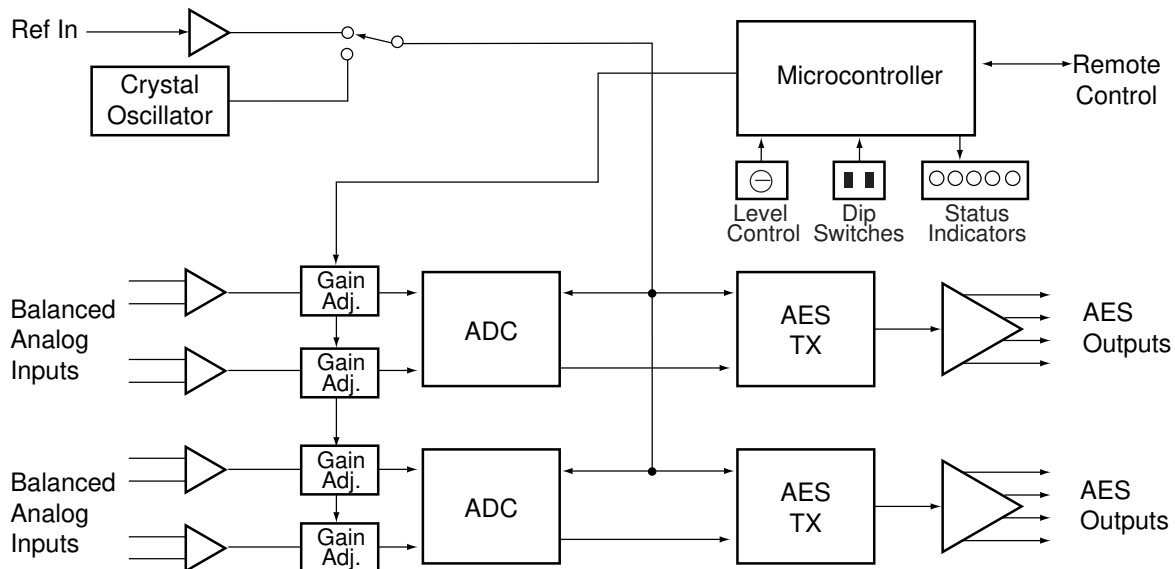
6010 Four Channel 20-bit Audio ADC Functional Block Diagram
