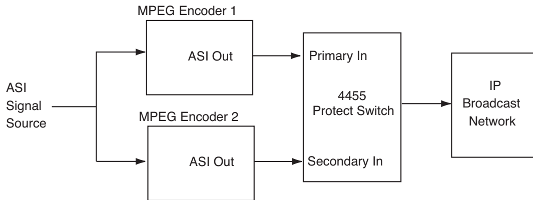
Redundant Auto-Switched Conversion With 4455 Module
