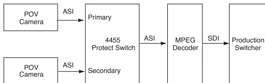
Signal Decision Maker With 4455 Module
